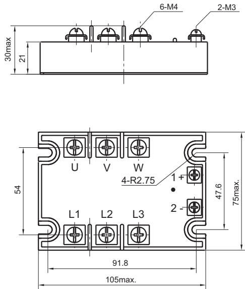
HFS24 (Non phase loss protection)
