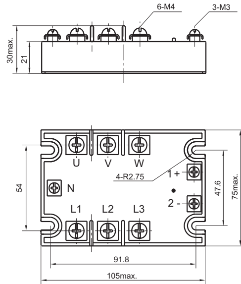
HFS24 (With phase loss protection)
