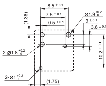
Single relay
