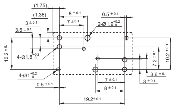
Twin relay
