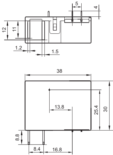
1 coil latching
