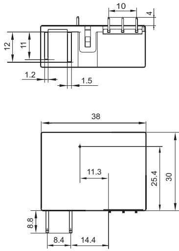
2 coils latching
